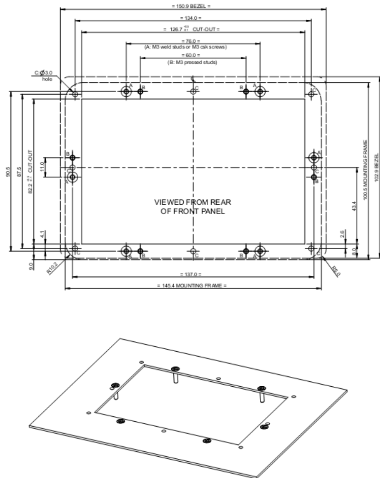
Figure 5.5 VM800P 5.0" panel mount dimensions
