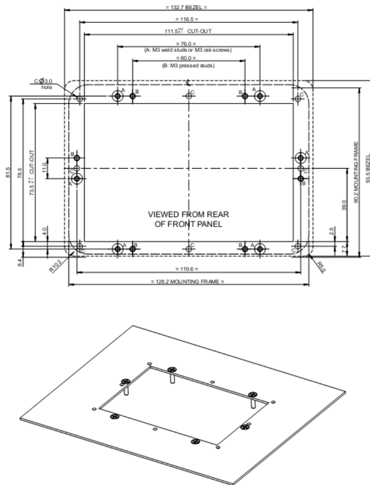
Figure 5.4 VM800P 4.3" panel mount dimensions
