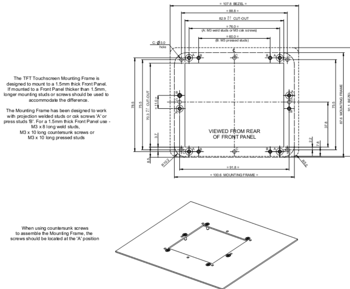
Figure 5.3 VM800P 3.5" panel mount dimensions
