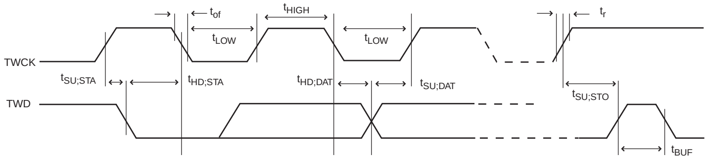
Figure 44-36. Two-wire Serial Bus Timing
