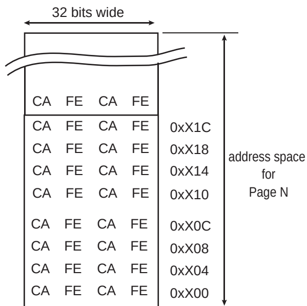
Figure 20-7. Full Page Programming
