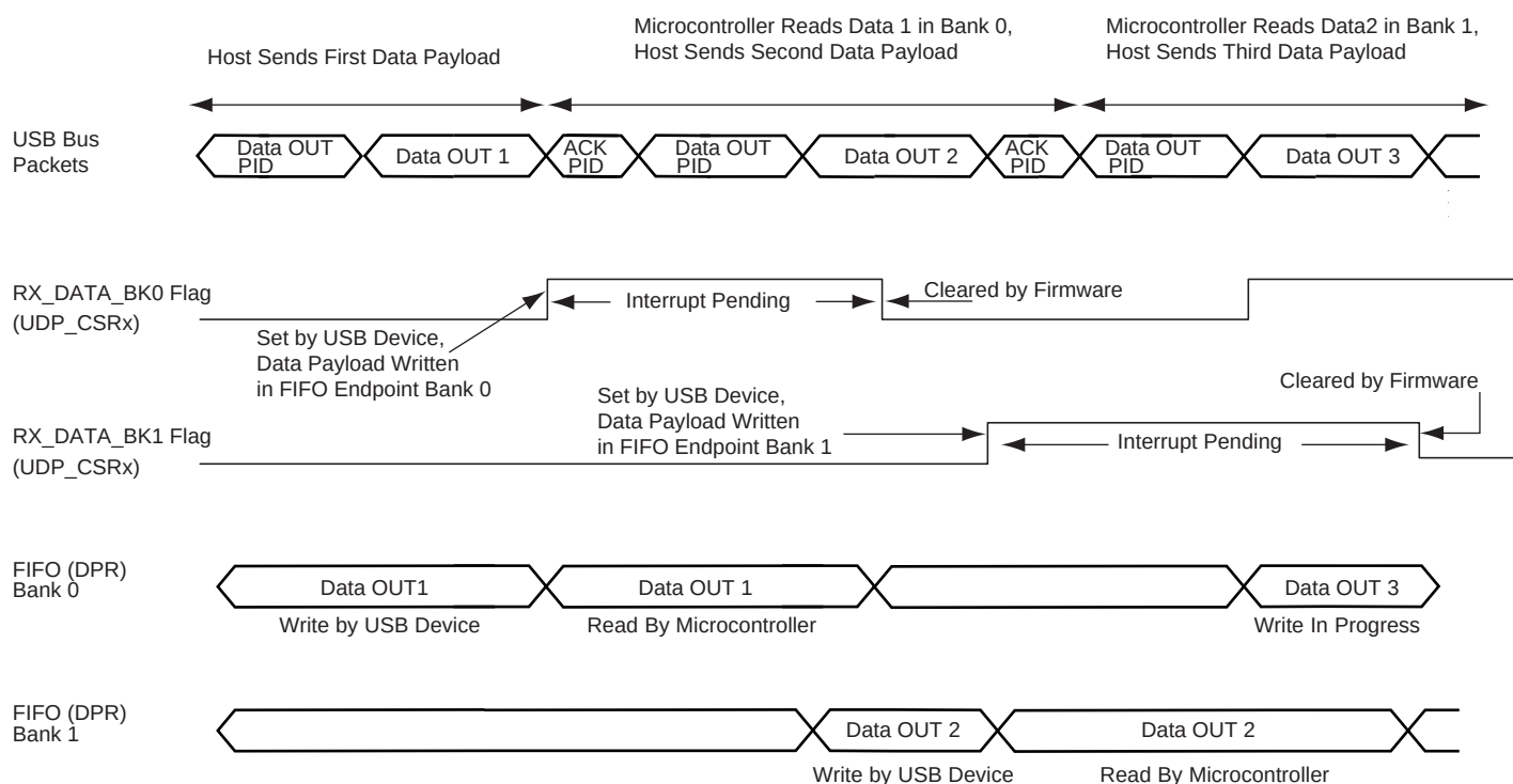
Figure 40-11. Data OUT Transfer for Ping-pong Endpoint
