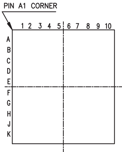
Figure 4-3. Orientation of the 100-ball VFBGA Package
