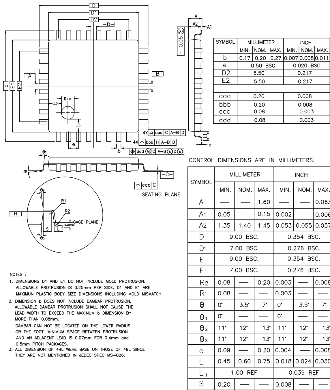
Figure 45-8. 48-lead LQFP Package Drawing
