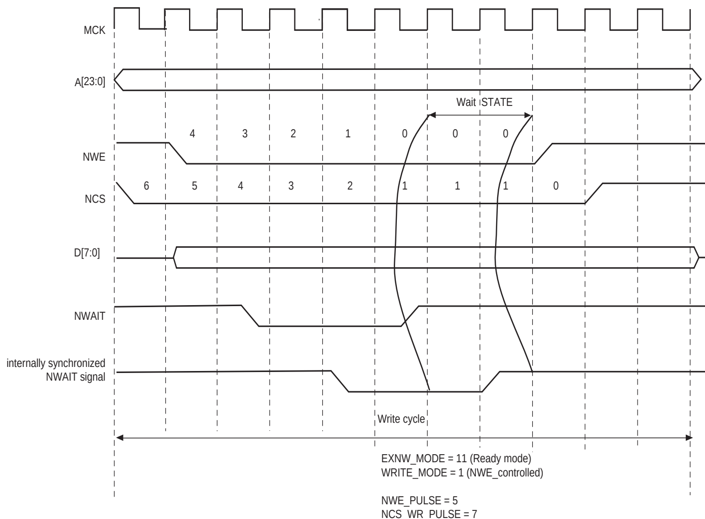
Figure 26-25. NWAIT Assertion in Write Access: Ready Mode ( \text{EXNW\_MODE} = 11 )
