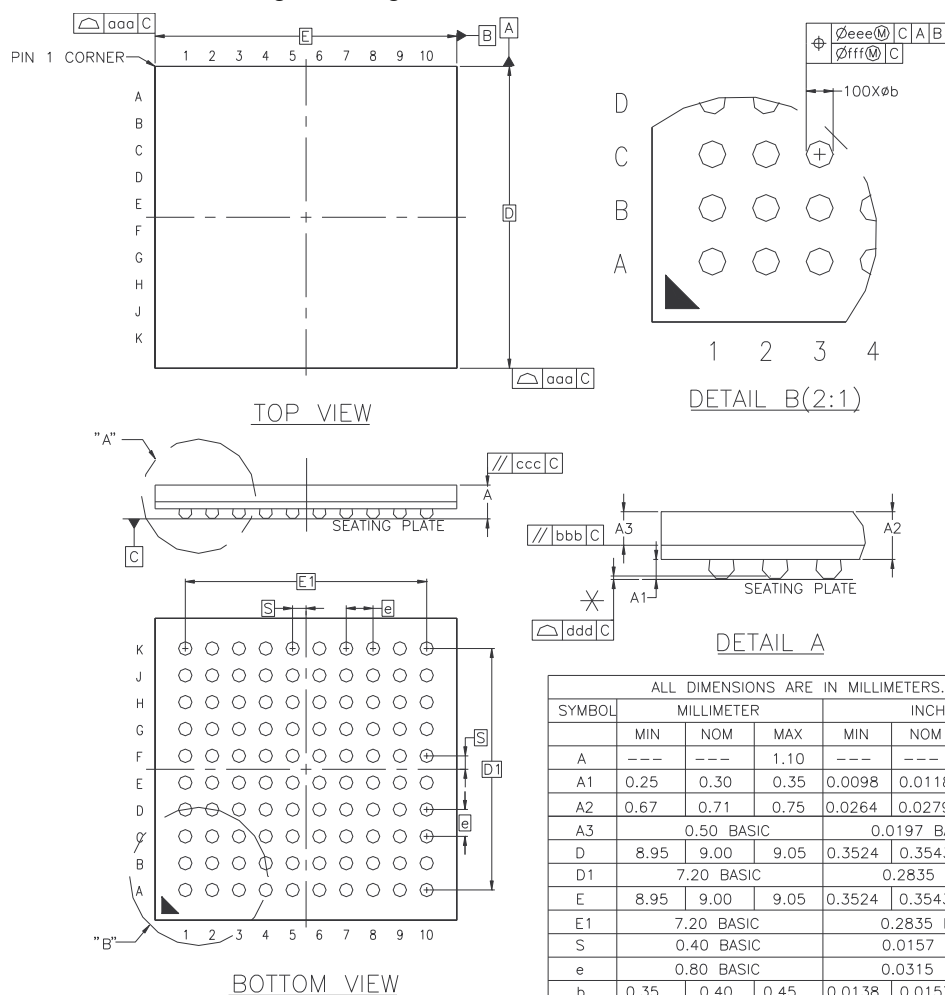
Figure 45-2. 100-ball TFBGA Package Drawing
