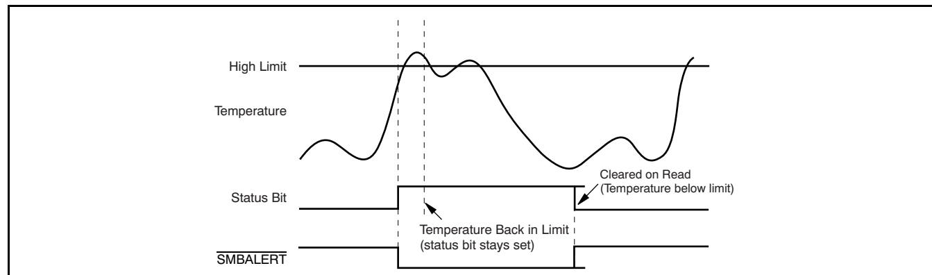
Figure 31. SMBALERT Pin and Status Bits Behavior
