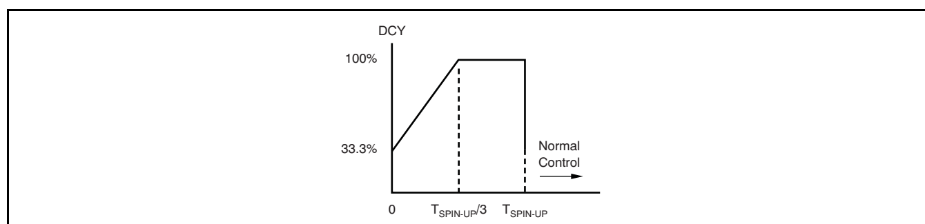
Figure 24. Spin-Up Process
