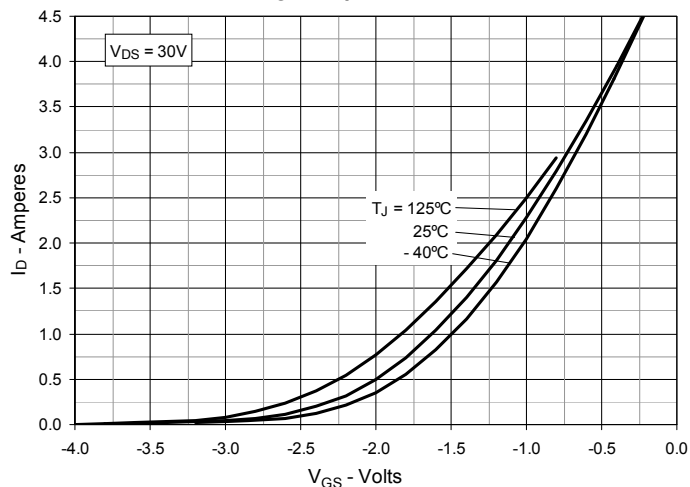
Fig. 9. Input Admittance
