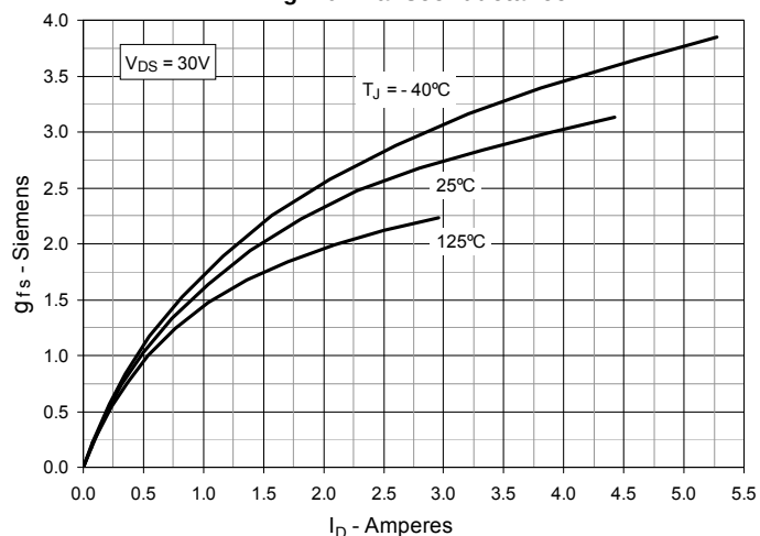
Fig. 10. Transconductance
