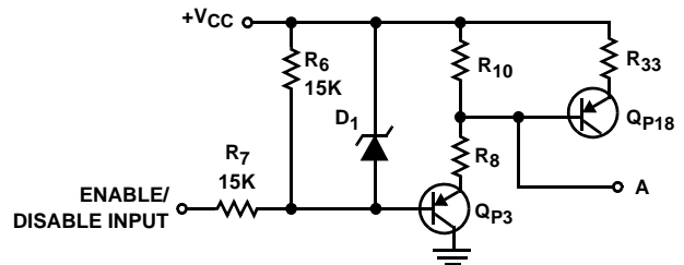
FIGURE 7. SIMPLIFIED SCHEMATIC OF ENABLE/DISABLE FUNCTION
