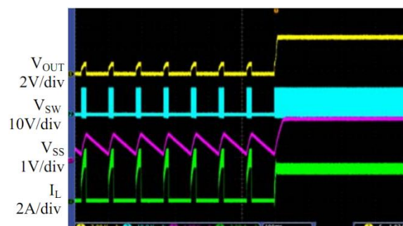
Time 100ms/div Fig. 15: Short-circuit recovery I_{OUT}=3A
