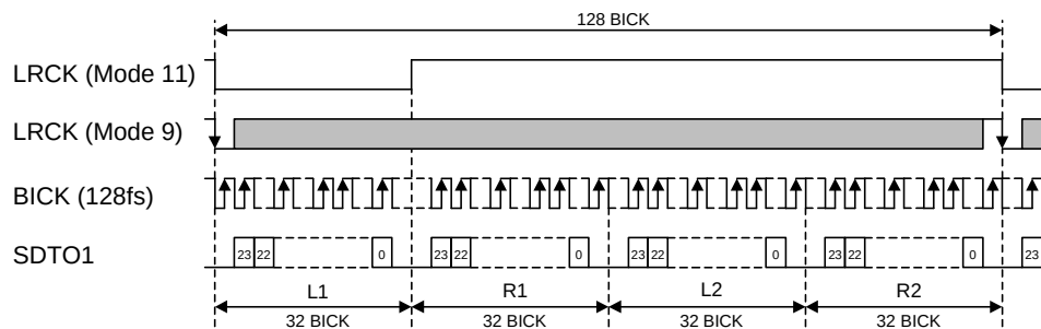
Figure 6. Mode 9, 11 Timing (TDM128 mode, I 2 S Compatible)
