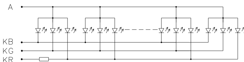
CIRCUIT DIAGRAM
