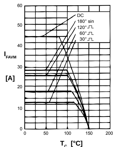
Fig. 3 Max. forward current at case temperature
