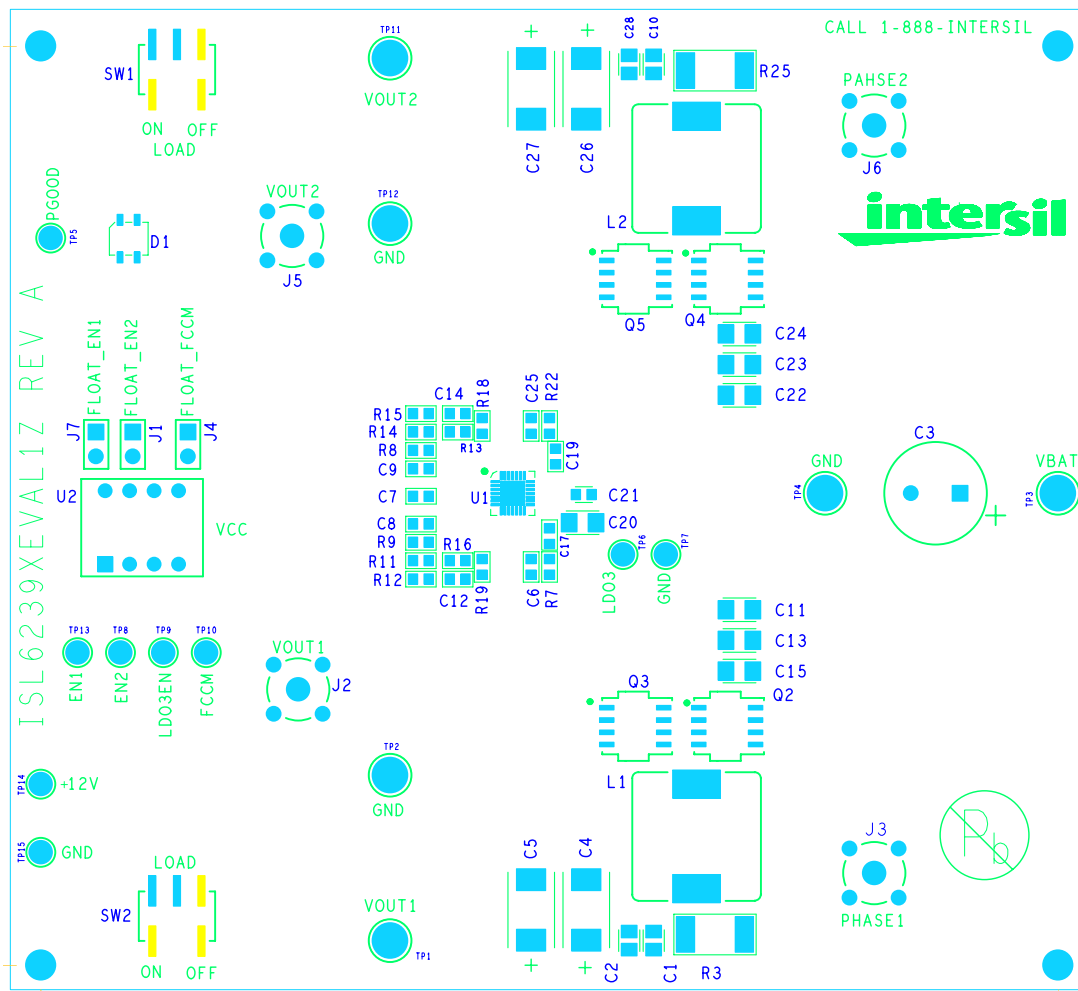
FIGURE 3. TOP SILKSCREEN
