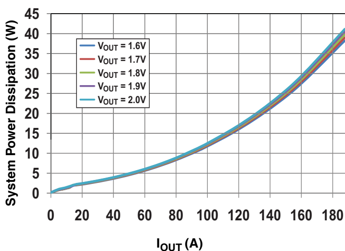
System Power Dissipation - 4 VT1697SB (VR12.5)
