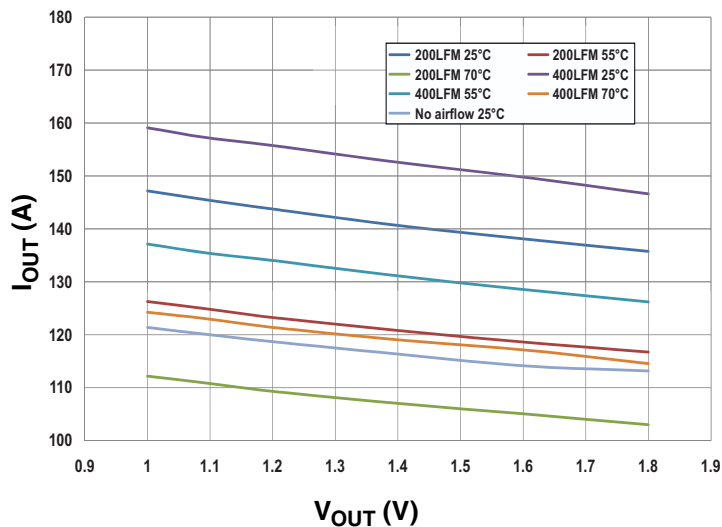
VT1697SB 4-Phase Safe Operating Area (No Heatsink)
