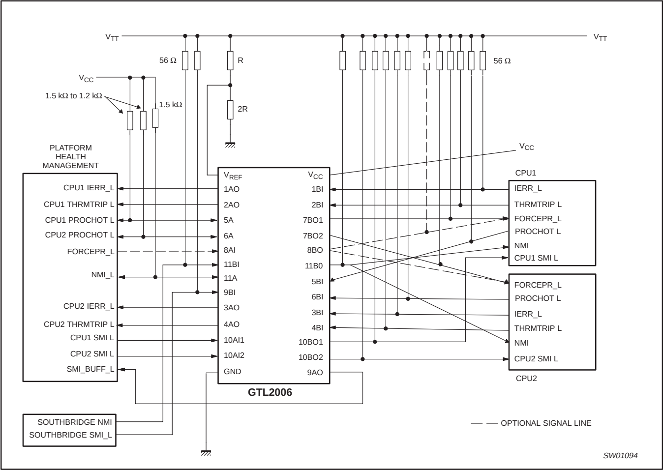
Figure 3. Application diagram
