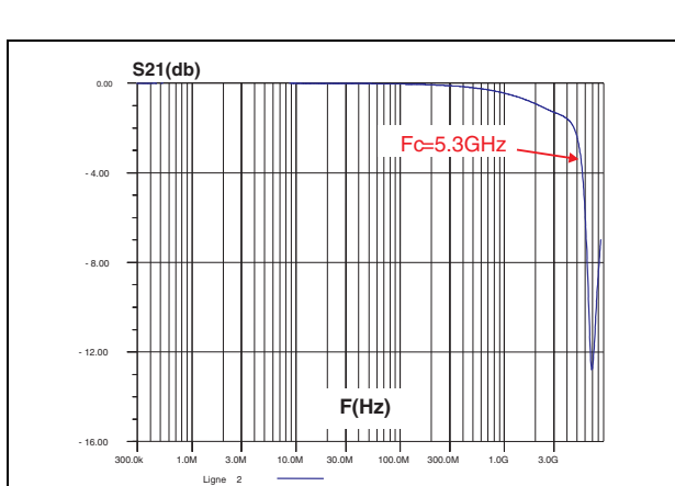
Figure 6. Frequency response (typical values) DVIULC6-2P6
