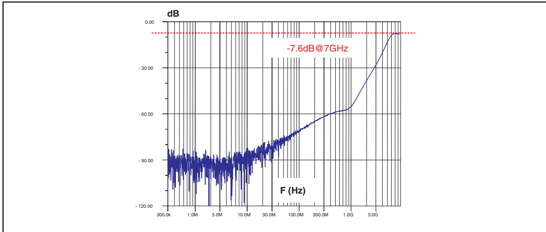
Figure 24. Analog crosstalk results (typical values) for DVIULC6-2M6
