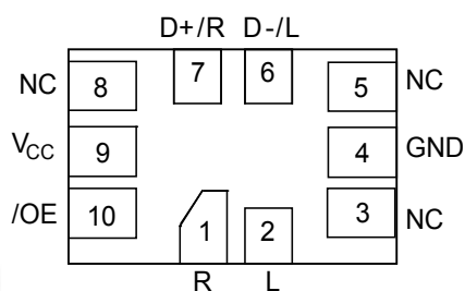
Figure 3. 10-Pin UMLP
