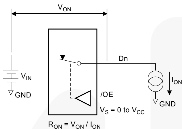
Figure 8. On Resistance
