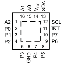
RGT PACKAGE (TOP VIEW)
