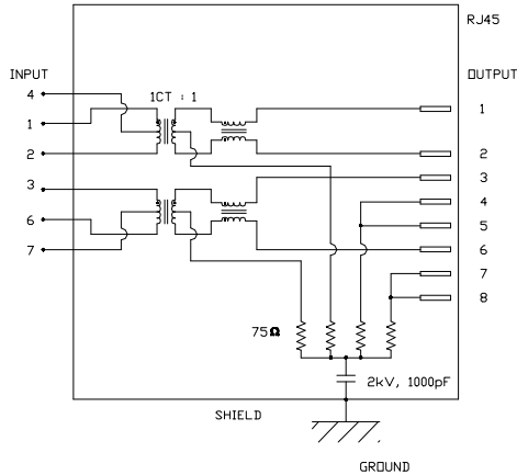
PACKAGE 24S3
