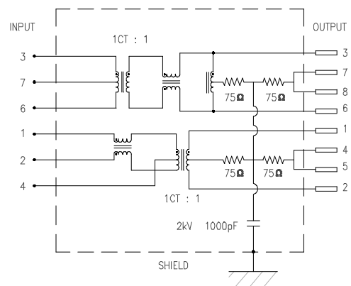
SCHEMATIC 14
