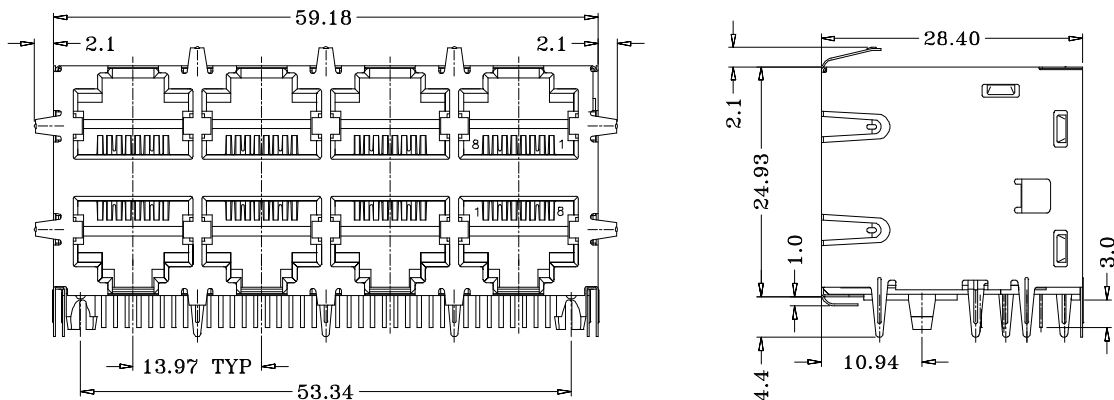
PACKAGE 24S3
