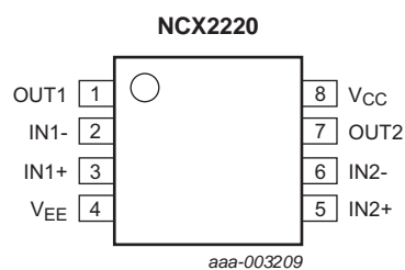
Fig 5. Pin configuration SOT505-2
