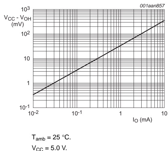
Fig 9. HIGH-level output voltage versus output current
