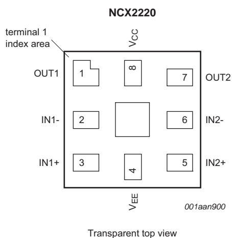
Fig 4. Pin configuration SOT902-2
