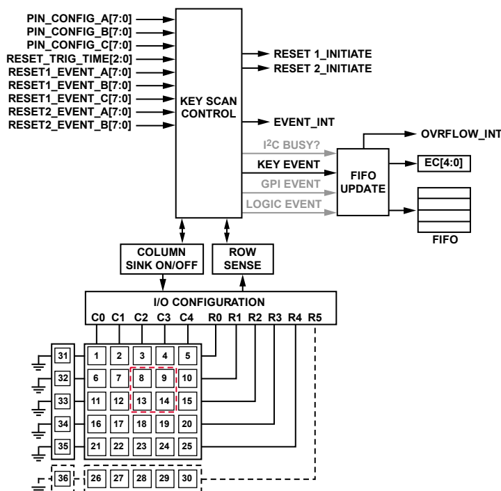
Figure 11. Detailed Key Scan Block
