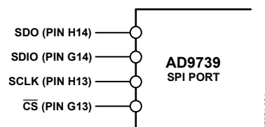
Figure 34. AD9739 SPI Port
