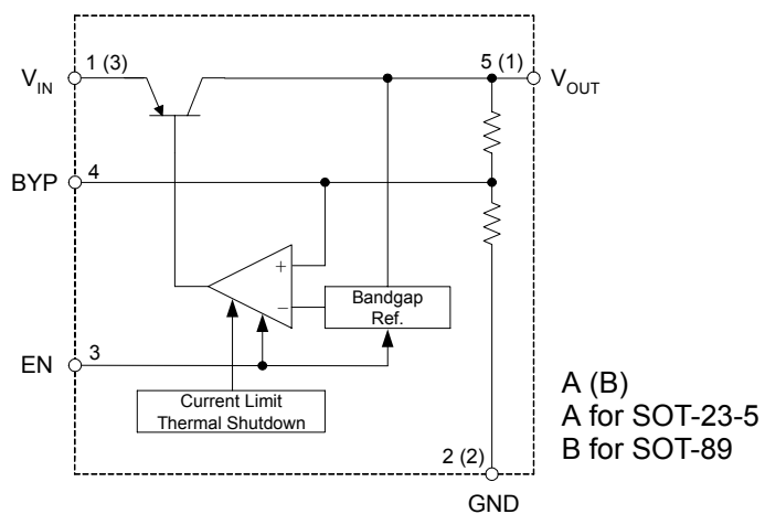
Fixed Regulator
