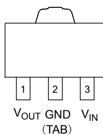
Figure 2. Pin Configuration of AP2202 (Top View)
