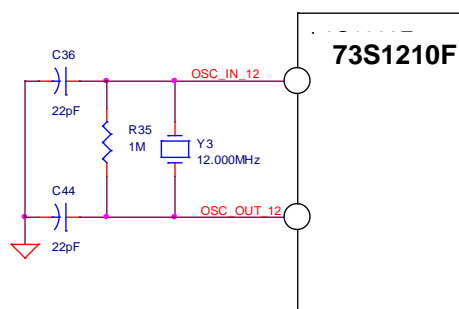
Figure 14: Oscillator Circuit
