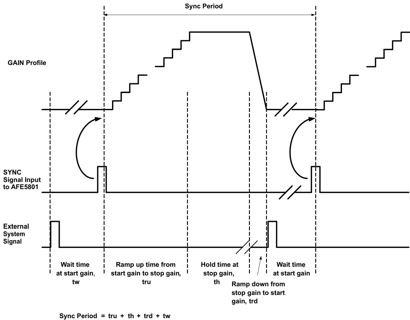
Figure 38. SYNC Period
