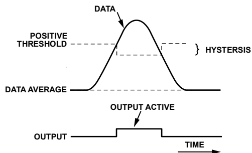
Figure 32. Threshold Hysteresis
