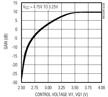
GAIN vs. CONTROL VOLTAGE (VI1 = VQ1)
