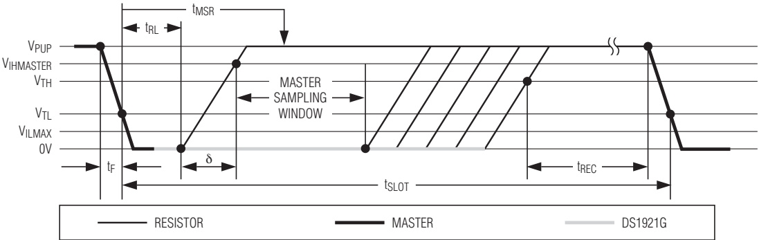
Figure 15. Read/Write Timing Diagram
