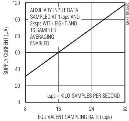
AVERAGE SUPPLY CURRENT vs. SAMPLING RATE
