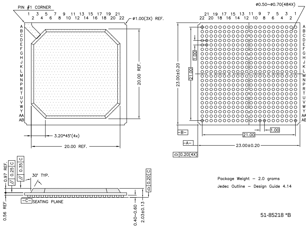
Figure 35. 484-ball PBGA (23 × 23 × 2.03 mm) BY484 Package Outline, 51-85218
