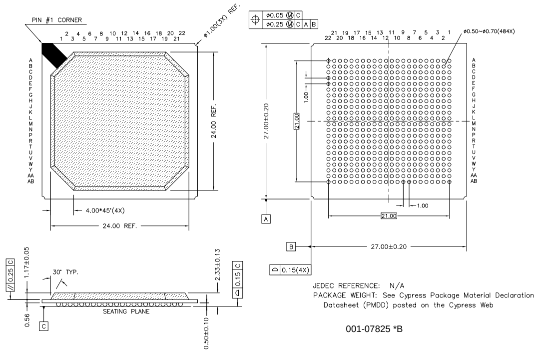
Figure 36. 484-ball PBGA (27 × 27 × 2.33 mm) BY484S Package Outline, 001-07825
