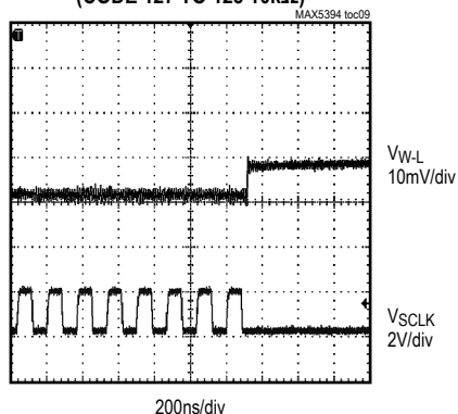
TAP-TO-TAP SWITCHING TRANSIENT (CODE 127 TO 128 10k \Omega )
