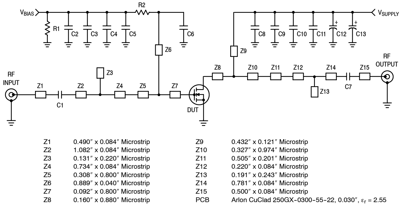
Figure 16. MRF7S19080HR3(HSR3) Test Circuit Schematic — TD-SCDMA
