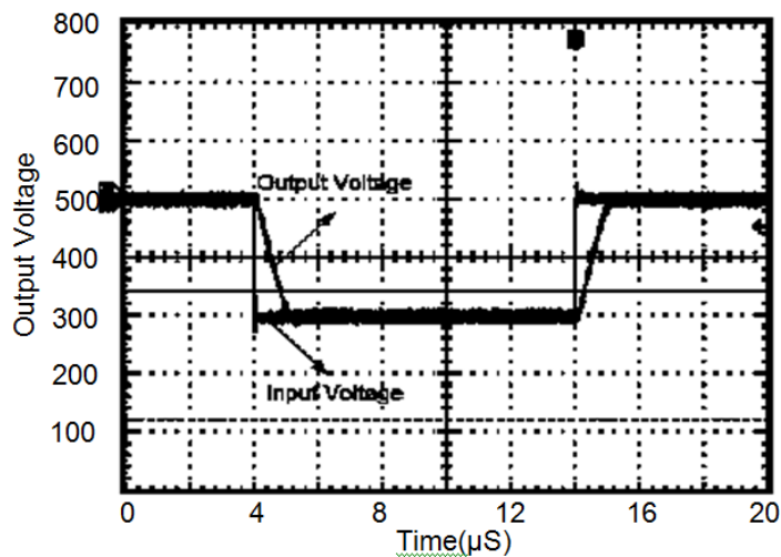
Voltage Follower Pulse Response (Small Signal)
