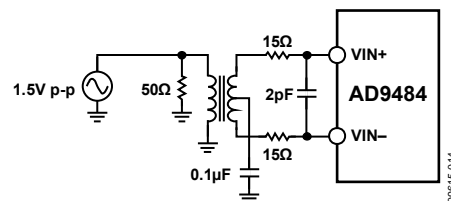
Figure 29. Differential Transformer—Coupled Configuration
