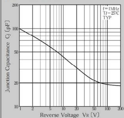
Junction Capacitance
