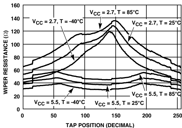
FIGURE 1. WIPER RESISTANCE vs TAP POSITION [ I(RW) = V_{CC}/R_{\text{TOTAL}} ] FOR 50k\Omega (U)
