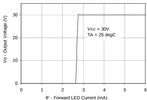
Figure 16: Transfer Characteristics
