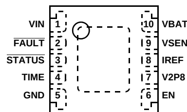
ISL6292C (3x3 DFN) TOP VIEW
