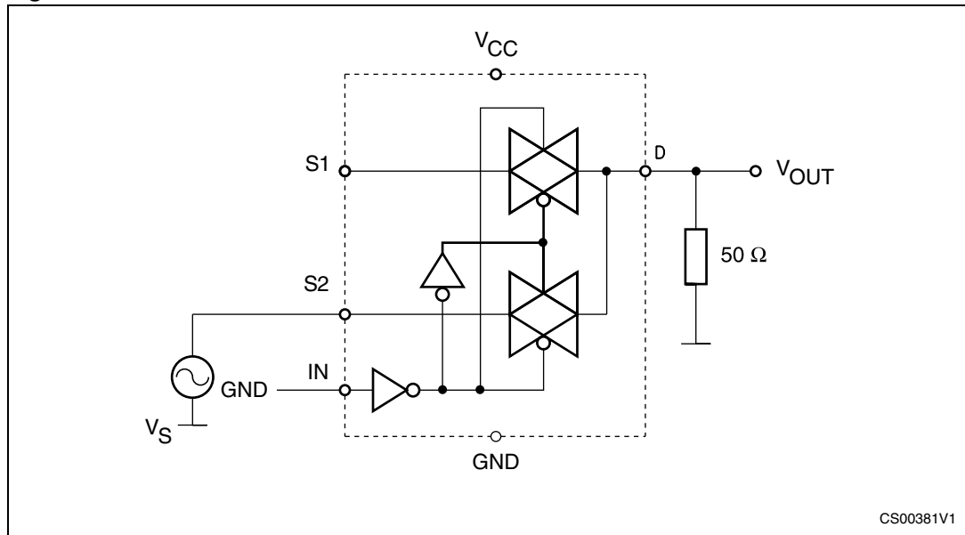
Figure 9. OFF isolation
