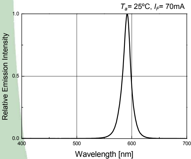
Spectrum
