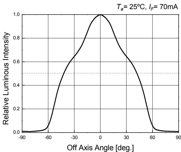
Directivity
