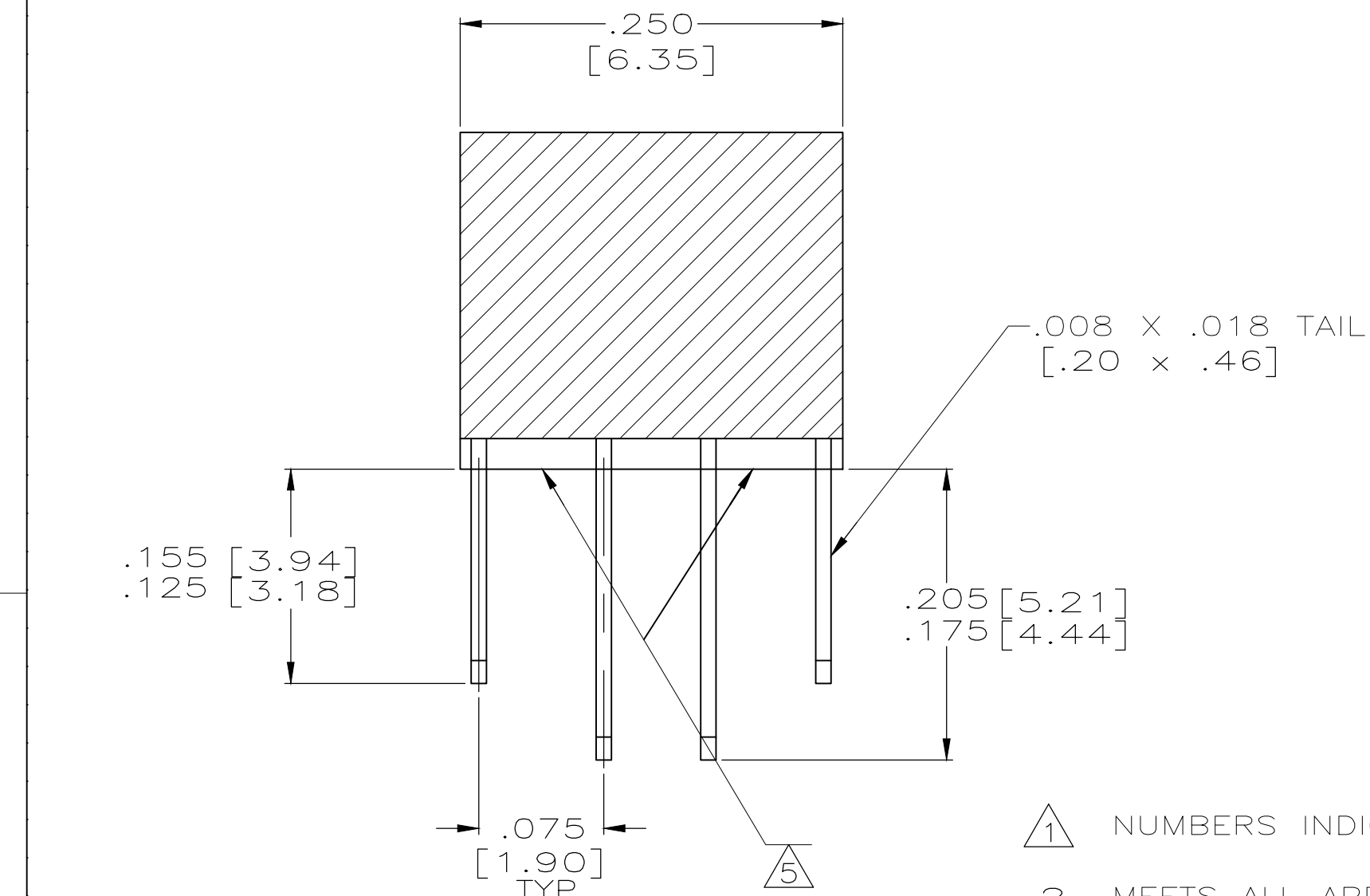
SECTION Z-Z SCALE 10:1
