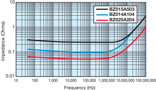
Impedance Comparison
