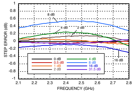
Step Error vs. Frequency
