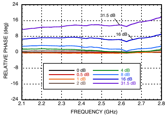
Relative Phase vs. Frequency
