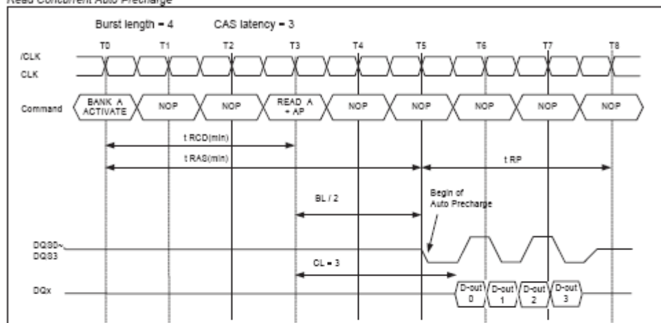
Read Concurrent Auto Precharge
