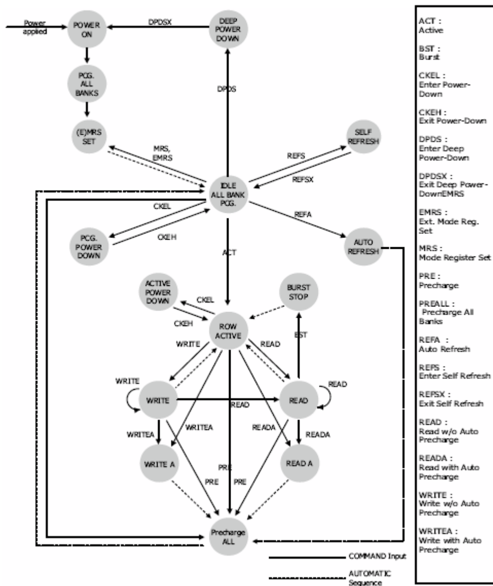
Mobile DDR SDRAM operation State Diagram
