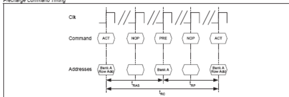
Precharge Command Timing
