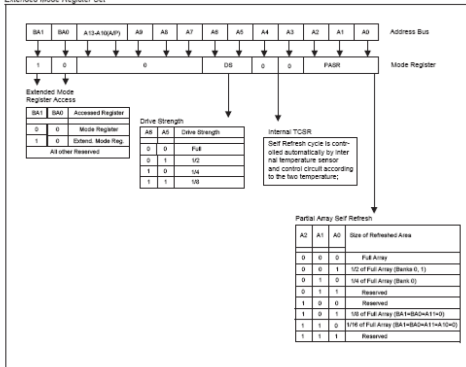
Extended Mode Register Set
