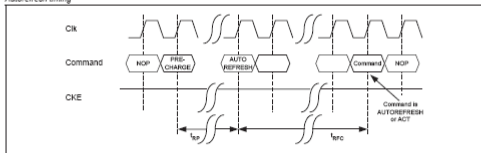
Autorefresh timing
