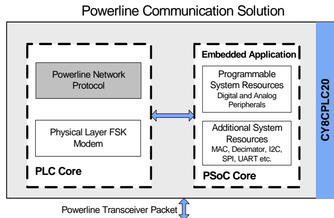
Figure 4. Powerline Network Protocol
