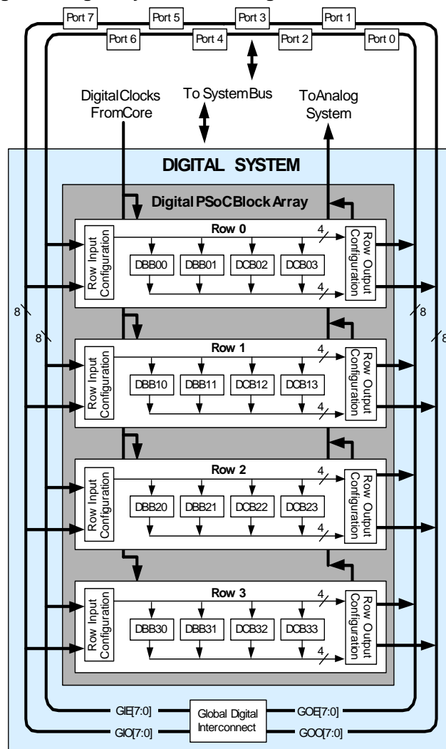
Figure 7. Digital System Block Diagram
