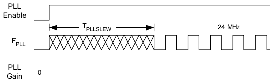
Figure 14. PLL Lock Timing Diagram
