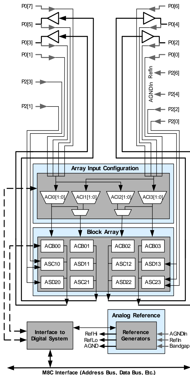
Figure 8. Analog System Block Diagram
