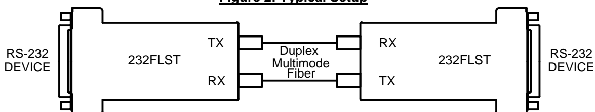
Figure 2: Typical Setup
