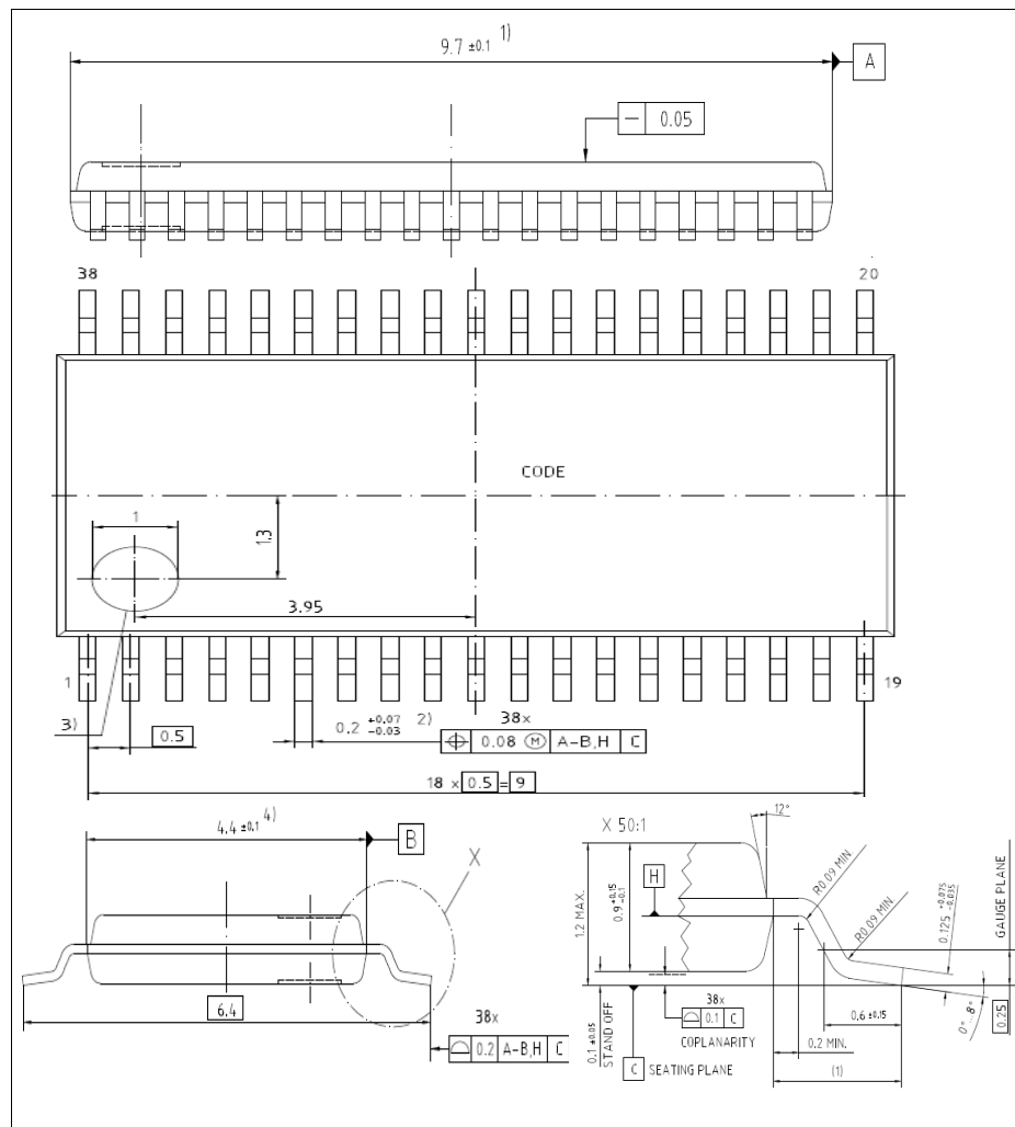
Figure 26 PG-TSSOP-38-9
