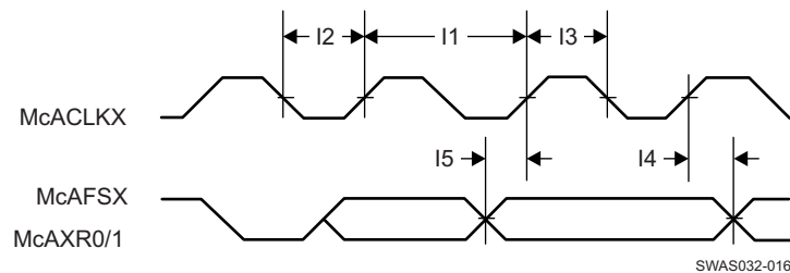
Figure 4-12. I2S Receive Mode Timing Diagram
