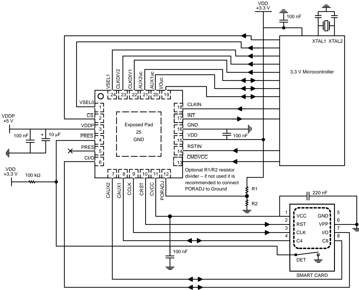
Figure 8. Application Schematic
