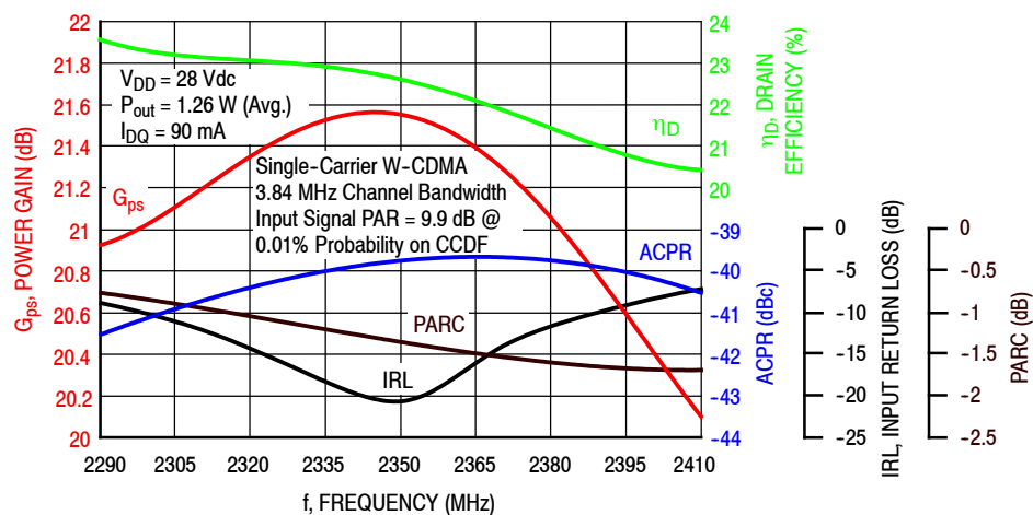
Figure 21. Single-Carrier Output Peak-to-Average Ratio Compression (PARC) Broadband Performance @ P_{out} = 1.26 \text{ W Avg.}
