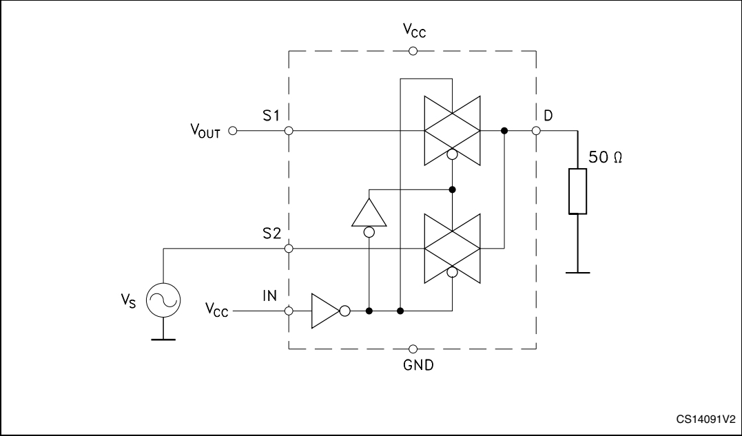
Figure 7. Channel-to-channel crosstalk
