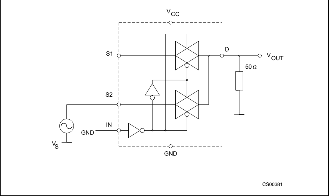
Figure 5. OFF isolation
