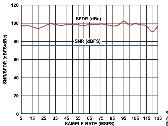
Figure 18. SNR/SFDR vs. Sample Rate with AIN = 9.7 MHz
