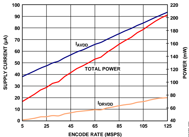
Figure 60. AD9648-125 Power and Current vs. Clock Rate (1.8 V CMOS Output Mode)
