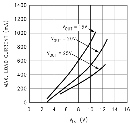
Figure 16. Max. Load Current vs V_{\text{IN}}
